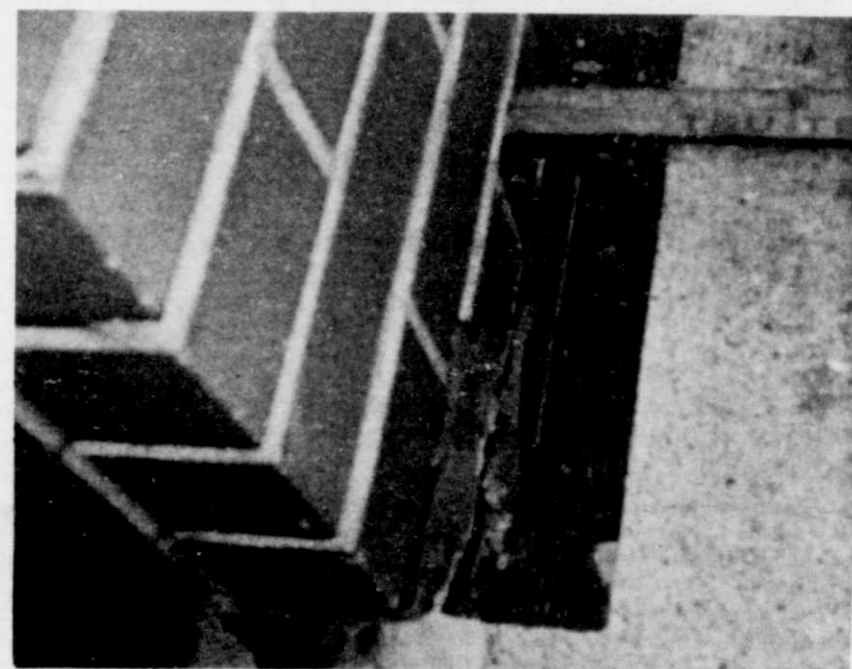
Beechwood Elementary — Concrete stoop pulled 3/4" away from building.
