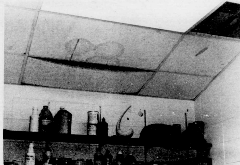
Kewaskum High School — Roof leaks. Water damage in art room. Another area to the right had 30 gallon pails under it to catch rain water.
