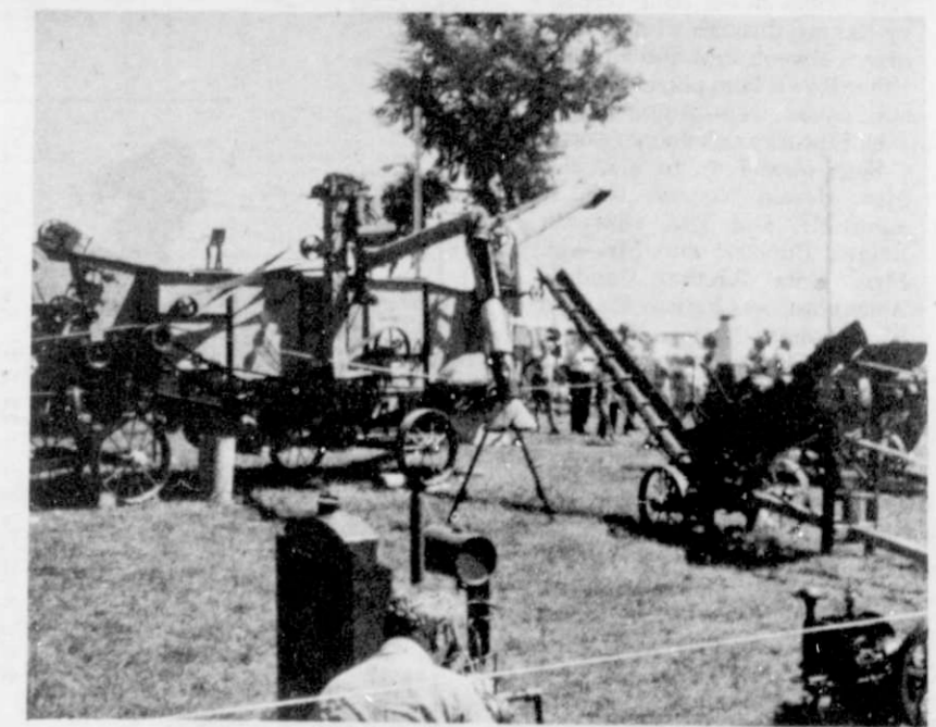
Old threshing machine and Rommel corn husker.
