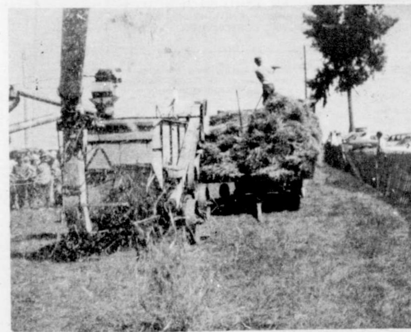
Old threshing machine in operation.
