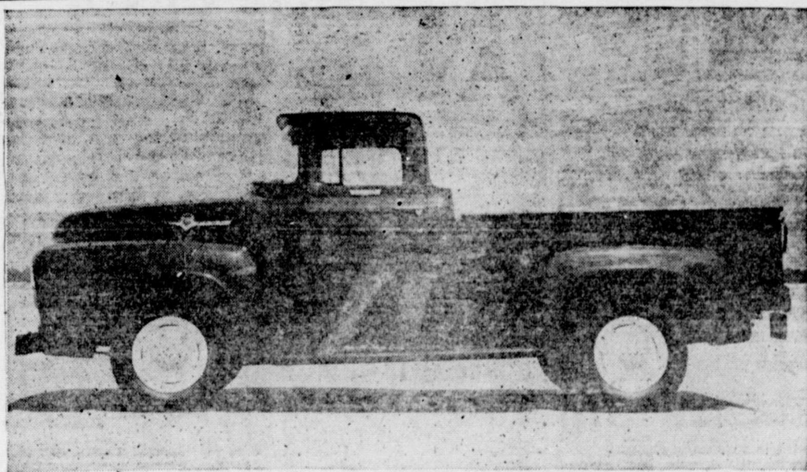
© NEW CAB STYLE—Ford's F-100 pickup truck with wraparound windshield and hooded roof is available in a 110 or 118 inch wheelbase to carry either a 45 or 65 cubic foot box. Powered by a 223 cu. in. I-block six cylinder engine rated at 133 hp, or a 272 cu. in. Y-8 rated at 167 hp, the pickup has five transmissions available: standard, overdrive, Fordomatic and heavy duty 3 speed and 4 speed.
